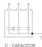
INNER CONNECTION
