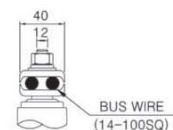
TERMINAL DETAIL
